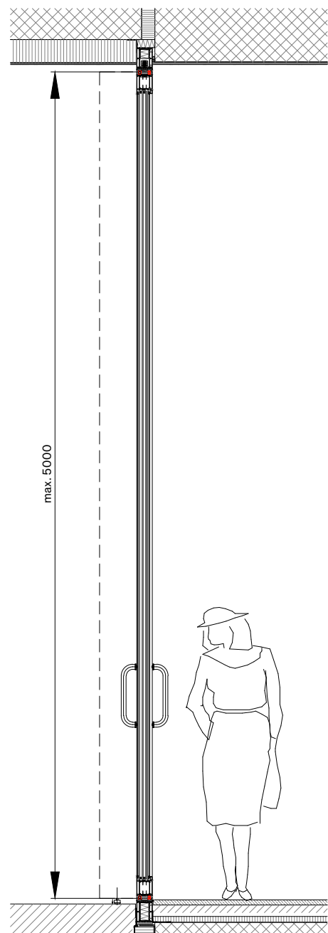
Vertical cross-section
